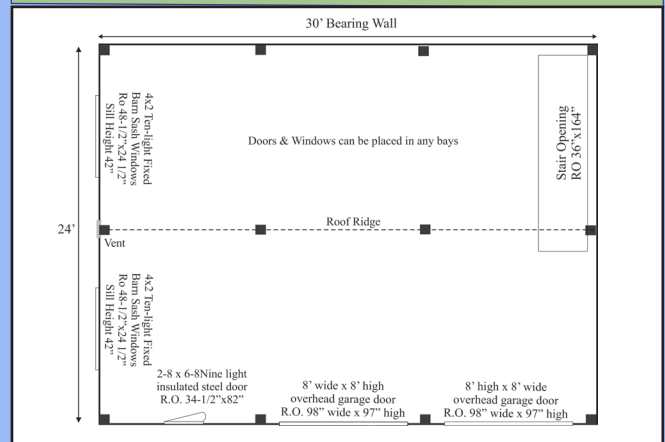
Floor Plan
