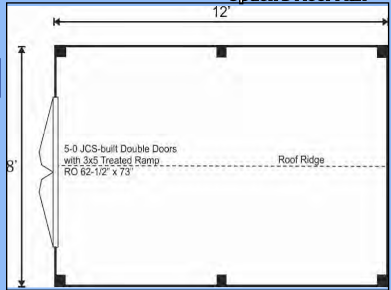
Option B Floor Plan
